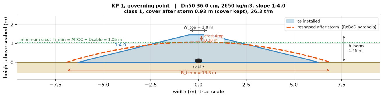
Figure 8.9: Cross-section of the optimised normal-density design at KP 1. The berm is built at 1.45 m and 26.2 tonnes per metre. It reshapes during the storm, the crest drops by 0.38 m and the toe spreads to 13.8 m, leaving 0.92 m of cover over the cable.
